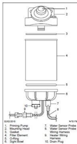
Fig. 1, Fuel/Water Separator Assembly
